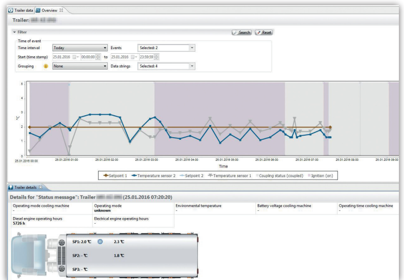
Cooling information and display of the cold chain in Trailer Data
